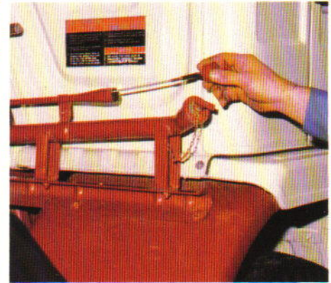
Regularly-checked items—like oil dipstick and windshield washer reservoir—are conveniently located outside so that routine maintenance can be accomplished without tilting the cab.
