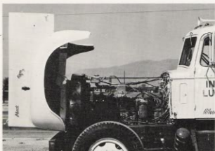
COMPLETE ACCESS — Clariben hoods offer immediate and complete access to the engine compartment. Service and overhaul downtime is drastically reduced.
