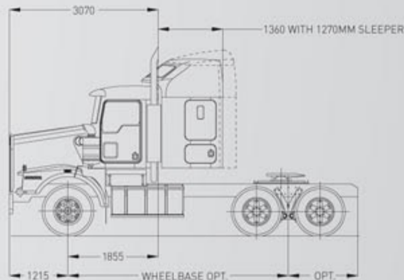
T659 1270MM SLEEPER BOX AERO II ROOF
