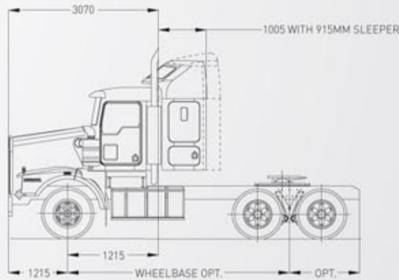
T659 915MM SLEEPER BOX AERO II ROOF
