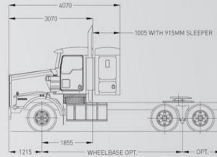
T659 915MM SLEEPER BOX FLAT ROOF
