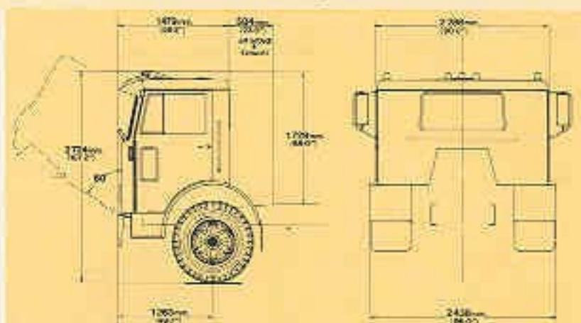
DIMENSIONS ARE IN MILLIMETRES AND (INCHES).
