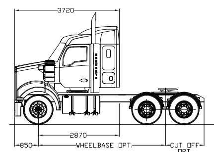
T610SAR 860MM SLEEPER
