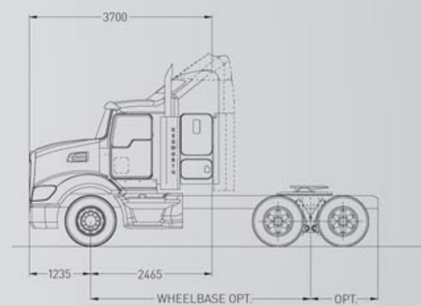
T403 36" RECESSED BACK SLEEPER
